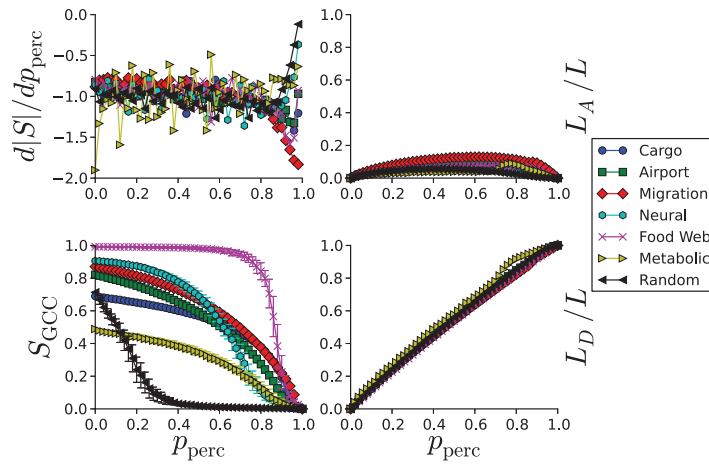
FIG. 7. Changes to the disparity backbone under link percolation. (top left) The size of the backbone is not robust to link percolation which is in contrast to the salience skeleton. (bottom left) In agreement with the salience skeleton, the GCC of the disparity backbone is also robust to link percolation, yet not quite to the same extent. (top right) Relatively few links are added to the disparity backbone as links are deleted. Again, this is in contrast to the salience skeleton where enough links were added to compensate for the links deleted from the skeleton. (bottom right) The rate at which links are deleted from the backbone is similar to that for the salience skeleton. The main difference, however, is that this removal of links is not compensated for by the addition of new links.
